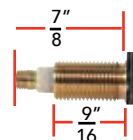
"X" Handshaft
