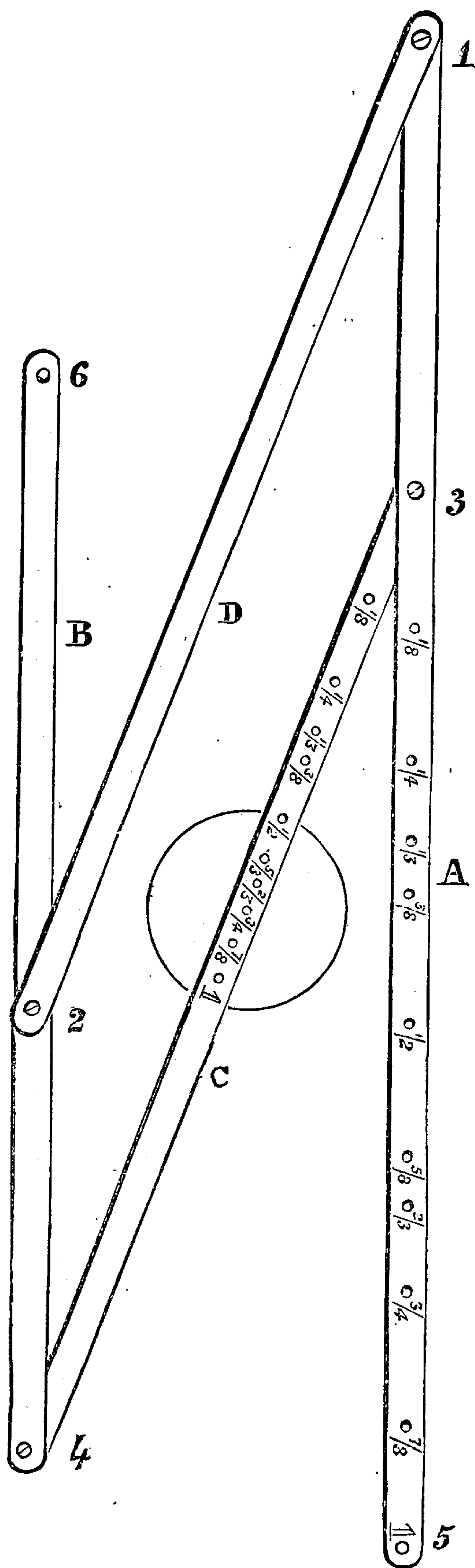
FIG. 43. THE PENTAGRAPH.
